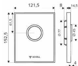
02 818 00 99, 02 819 00 99 Escudos Ambition cristal 02 826 00 99, 02 827 00 99 Ambition ECO cristal
